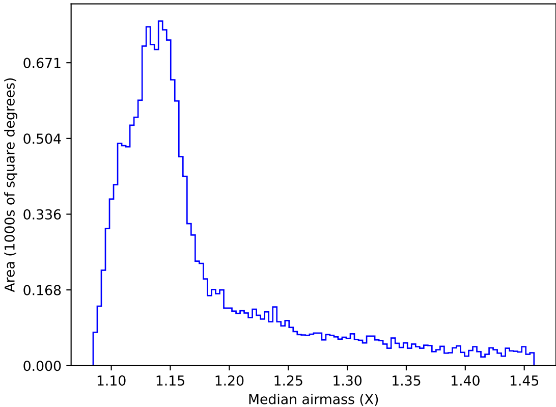
roll_pause_mjdp60_v3.4_10yrs WFD all bands: Median airmass
