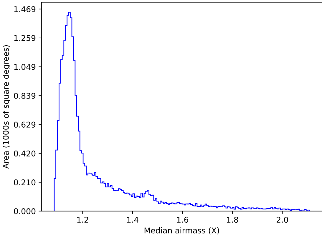
roll_pause_mjdp60_v3.4_10yrs All sky z band: Median airmass
