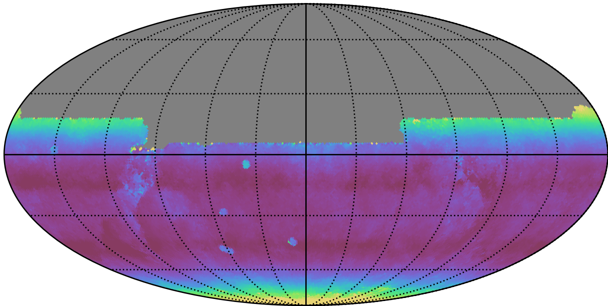
roll_pause_mjdp60_v3.4_10yrs All sky y band: Median airmass
