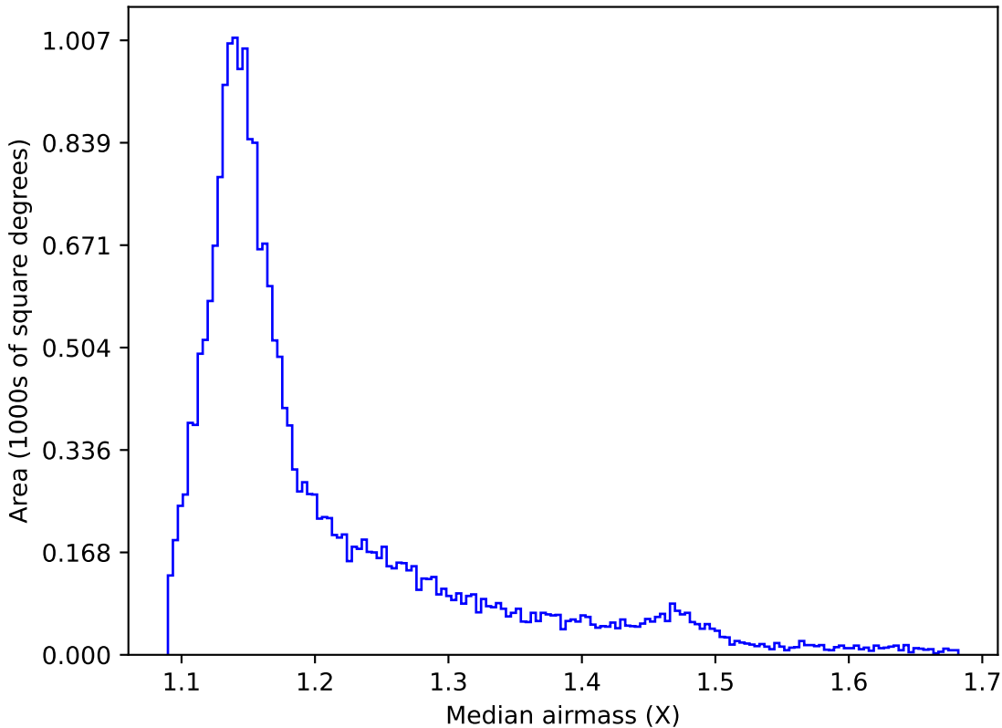
roll_pause_mjdp60_v3.4_10yrs All sky y band: Median airmass
