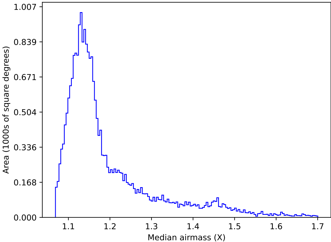
roll_pause_mjdp60_v3.4_10yrs All sky u band: Median airmass
