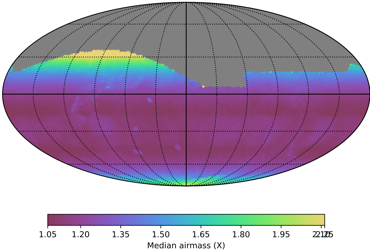
roll_pause_mjdp60_v3.4_10yrs All sky r band: Median airmass
