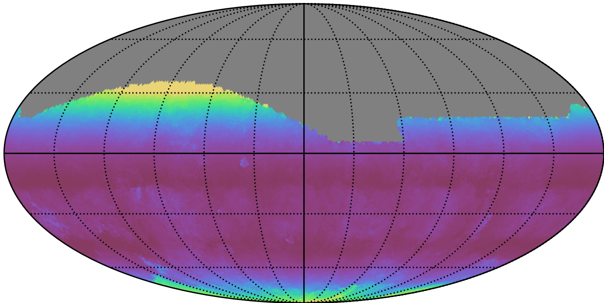
roll_pause_mjdp60_v3.4_10yrs All sky g band: Median airmass
