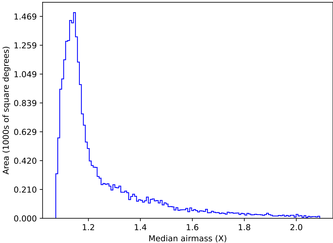
roll_pause_mjdp60_v3.4_10yrs All sky g band: Median airmass
