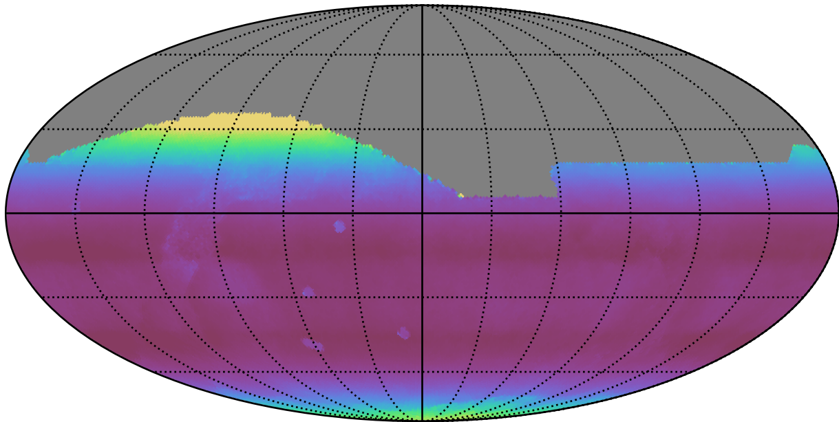
roll_pause_mjdp60_v3.4_10yrs All sky all bands: Median airmass
