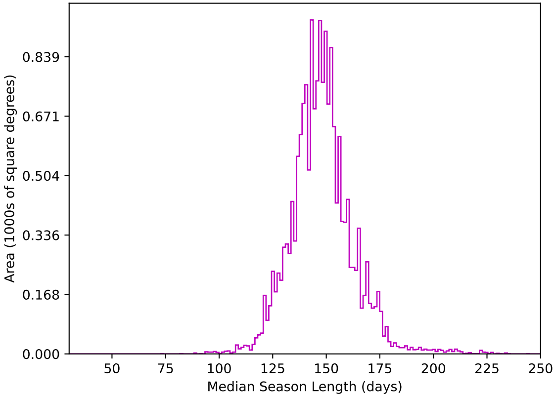
roll_pause_mjdp60_v3.4_10yrs WFD z band: Median Season Length
