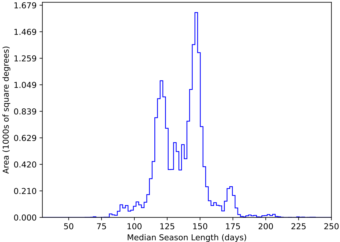
roll_pause_mjdp60_v3.4_10yrs WFD y band: Median Season Length
