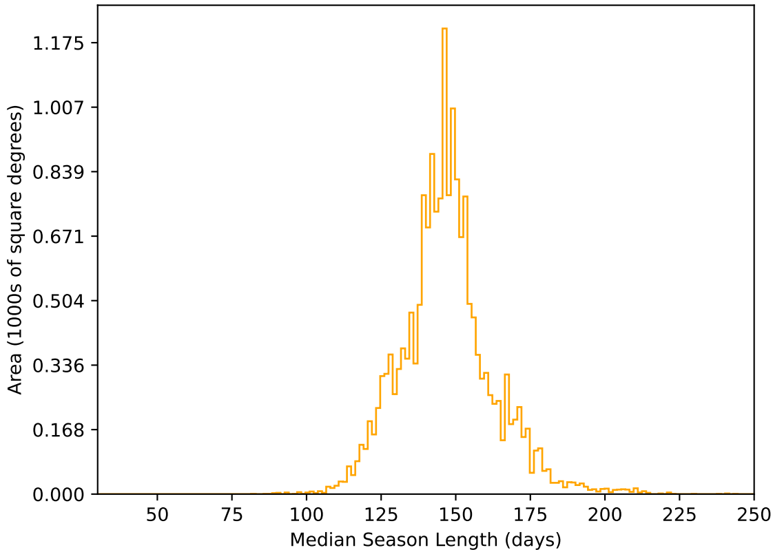
roll_pause_mjdp60_v3.4_10yrs WFD r band: Median Season Length
