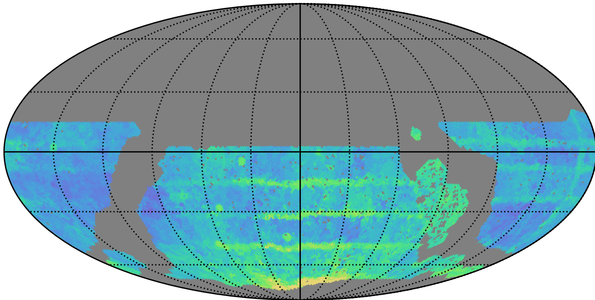
roll_pause_mjdp60_v3.4_10yrs WFD all bands: Median Season Length
