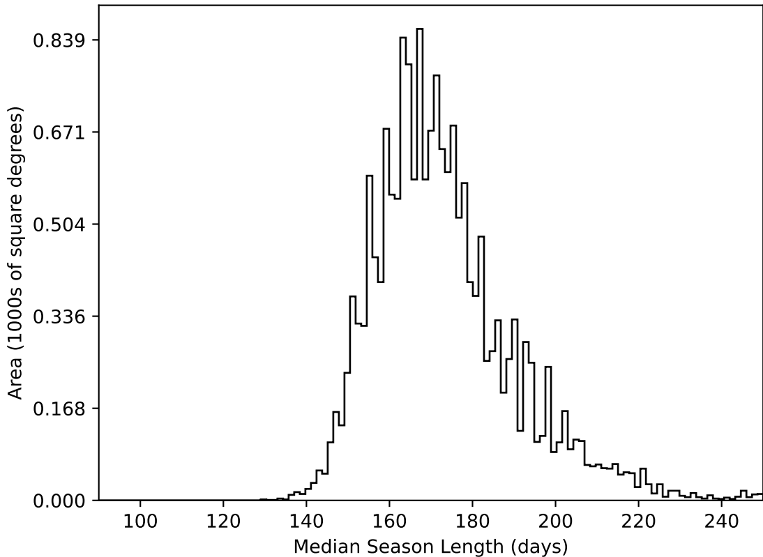
roll_pause_mjdp60_v3.4_10yrs WFD all bands: Median Season Length
