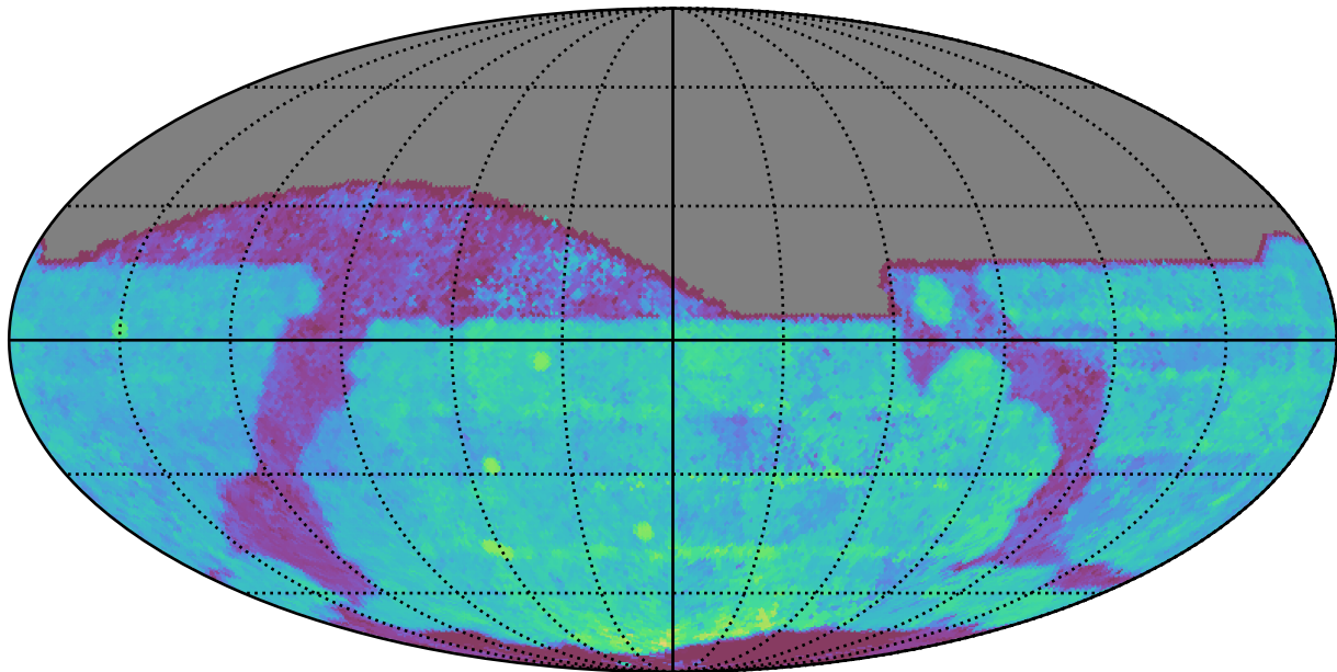
roll_pause_mjdp60_v3.4_10yrs All sky z band: Median Season Length
