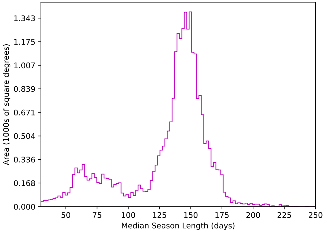
roll_pause_mjdp60_v3.4_10yrs All sky z band: Median Season Length
