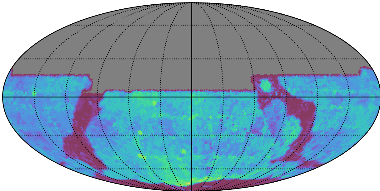
roll_pause_mjdp60_v3.4_10yrs All sky y band: Median Season Length
