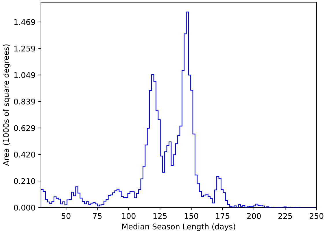
roll_pause_mjdp60_v3.4_10yrs All sky y band: Median Season Length
