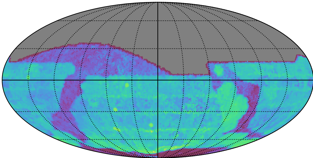
roll_pause_mjdp60_v3.4_10yrs All sky r band: Median Season Length
