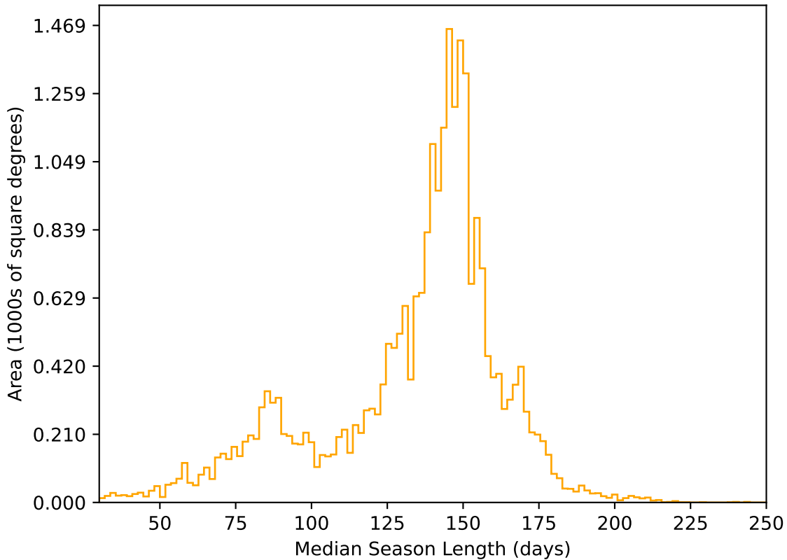
roll_pause_mjdp60_v3.4_10yrs All sky r band: Median Season Length
