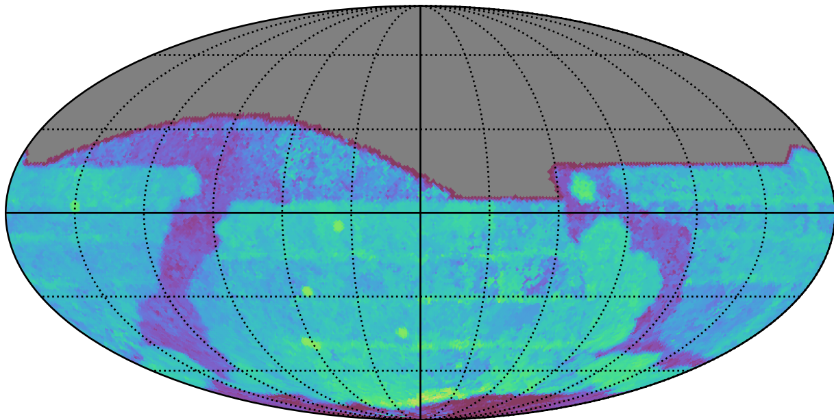
roll_pause_mjdp60_v3.4_10yrs All sky i band: Median Season Length
