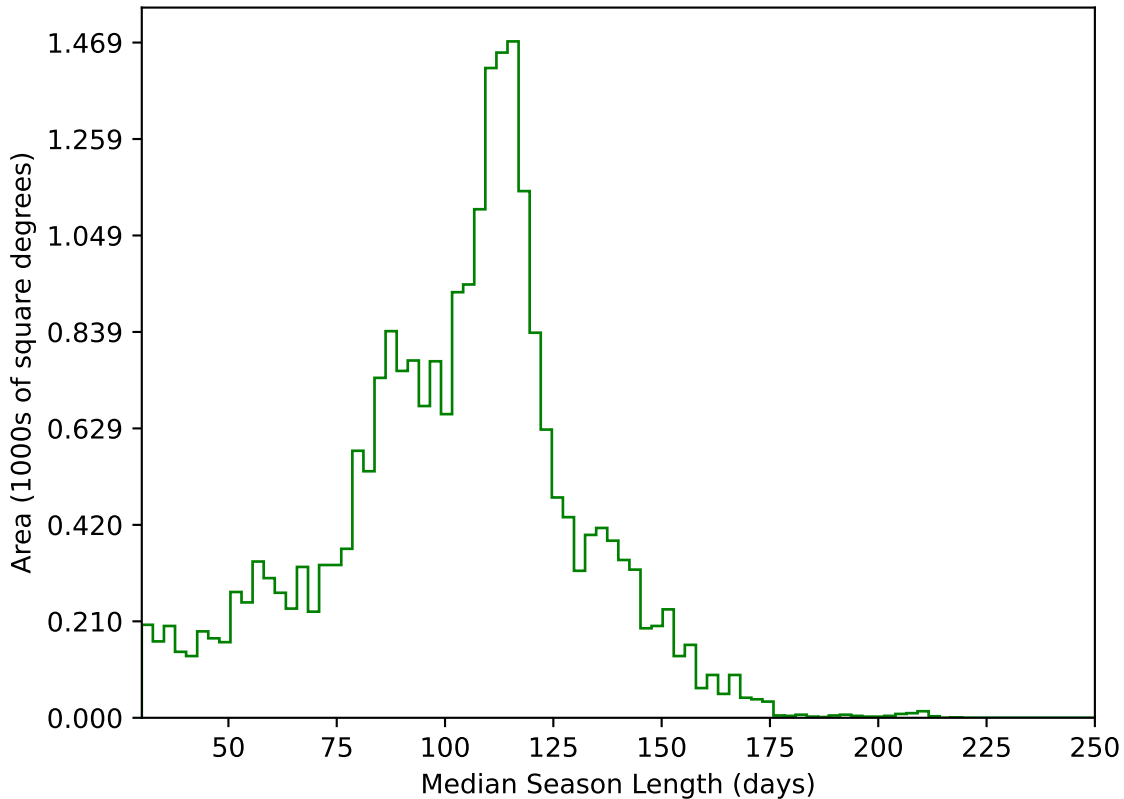
roll_pause_mjdp60_v3.4_10yrs All sky g band: Median Season Length
