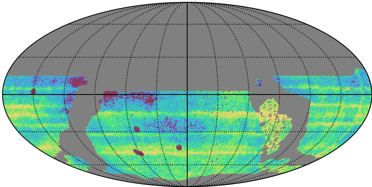
roll_pause_mjdp60_v3.4_10yrs WFD: Median Intra-Night Gap
