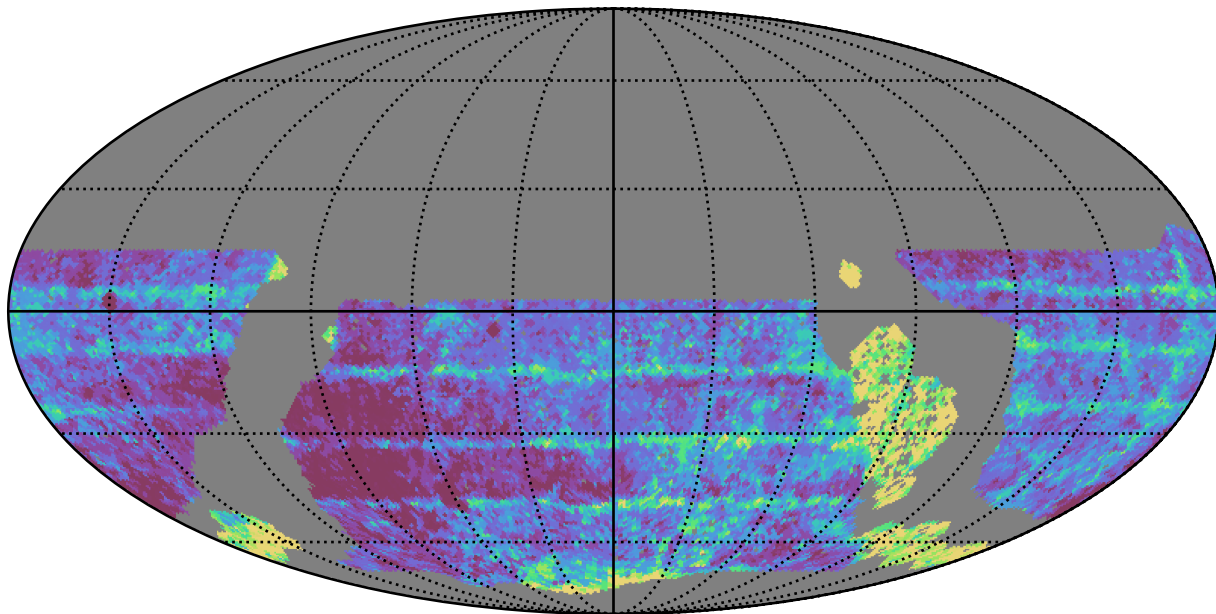
roll_pause_mjdp60_v3.4_10yrs WFD z band: Median Inter-Night Gap
