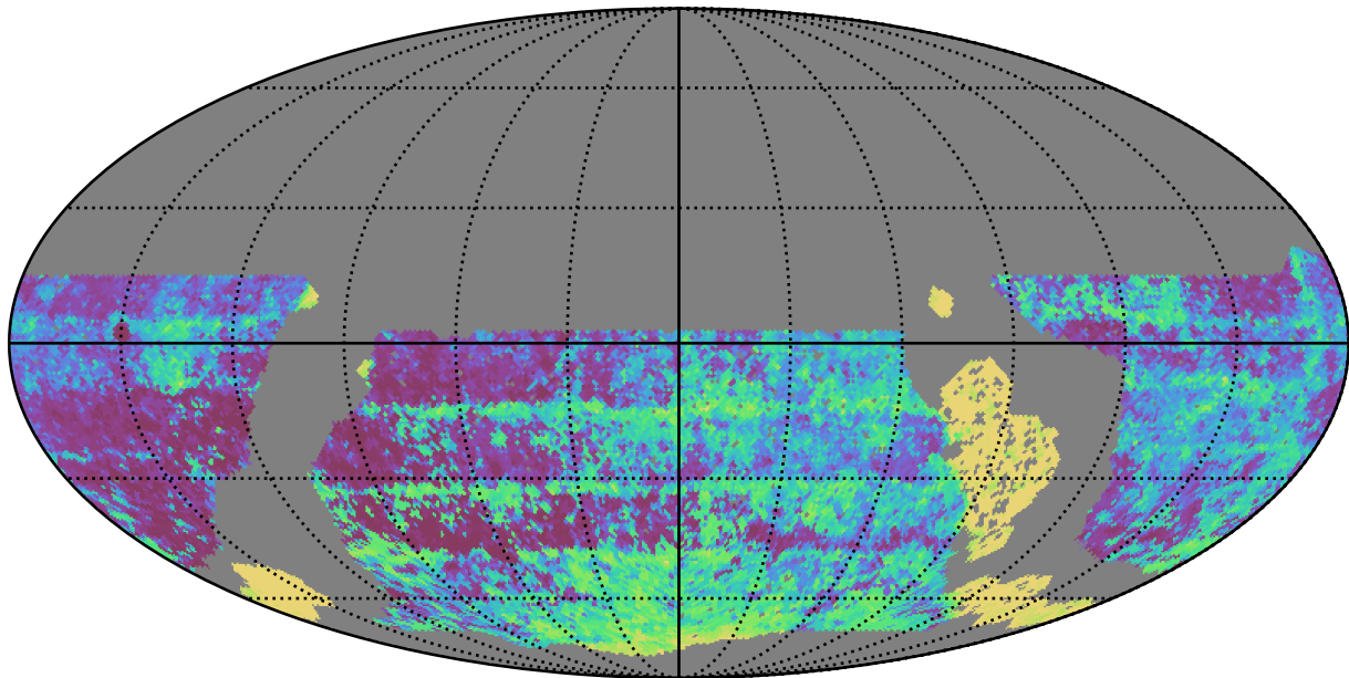
roll_pause_mjdp60_v3.4_10yrs WFD y band: Median Inter-Night Gap
