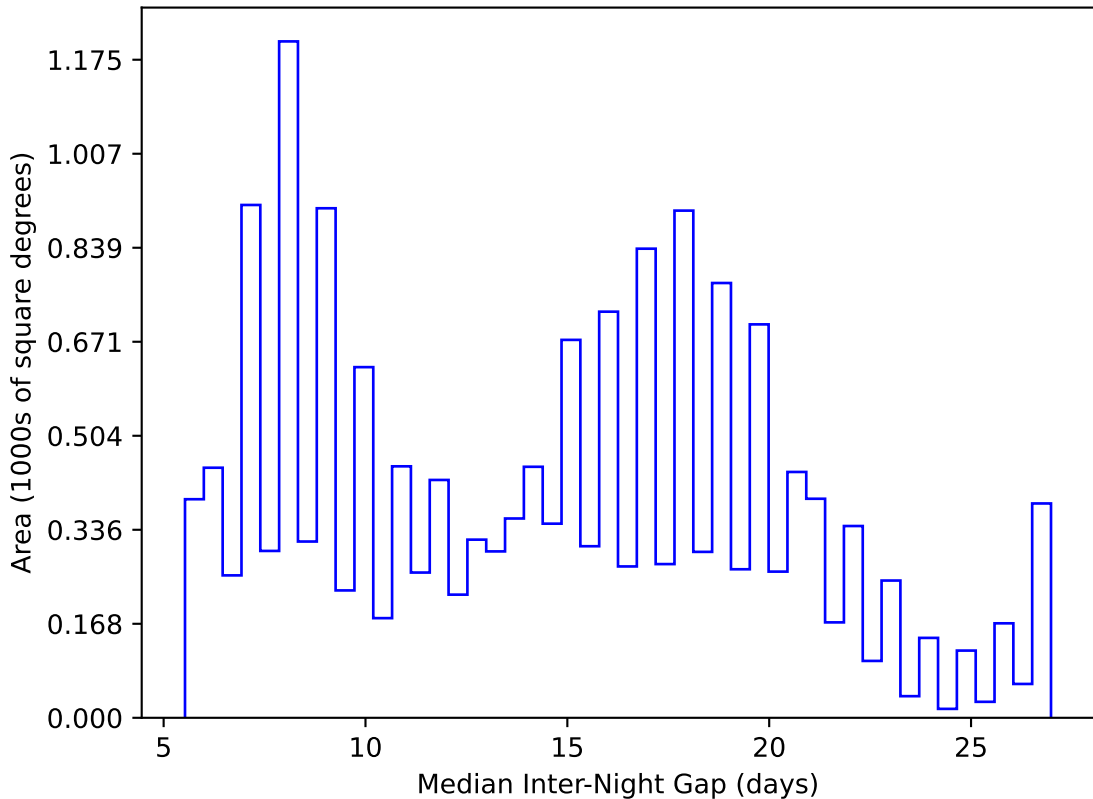
roll_pause_mjdp60_v3.4_10yrs WFD y band: Median Inter-Night Gap
