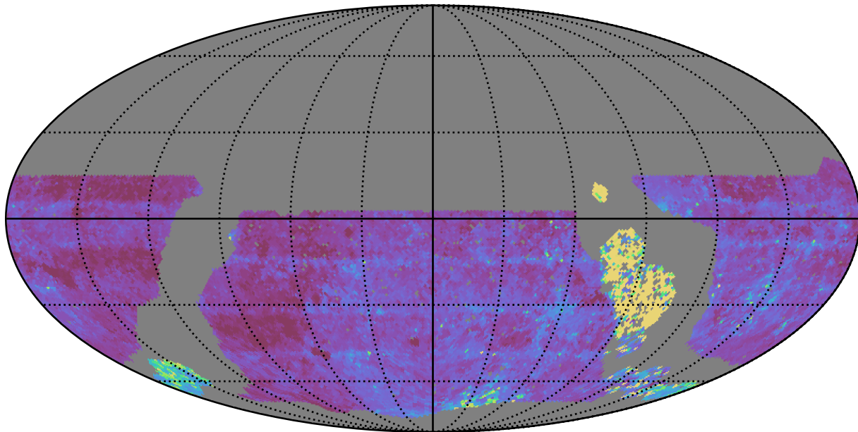
roll_pause_mjdp60_v3.4_10yrs WFD u band: Median Inter-Night Gap
