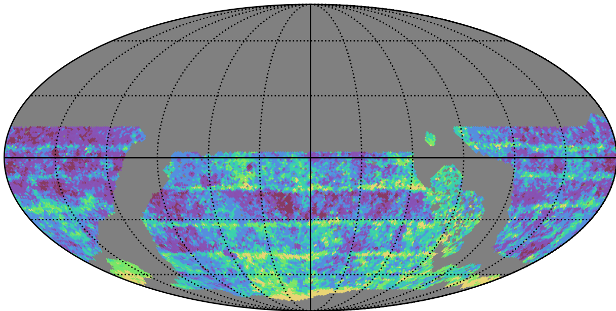
roll_pause_mjdp60_v3.4_10yrs WFD r band: Median Inter-Night Gap
