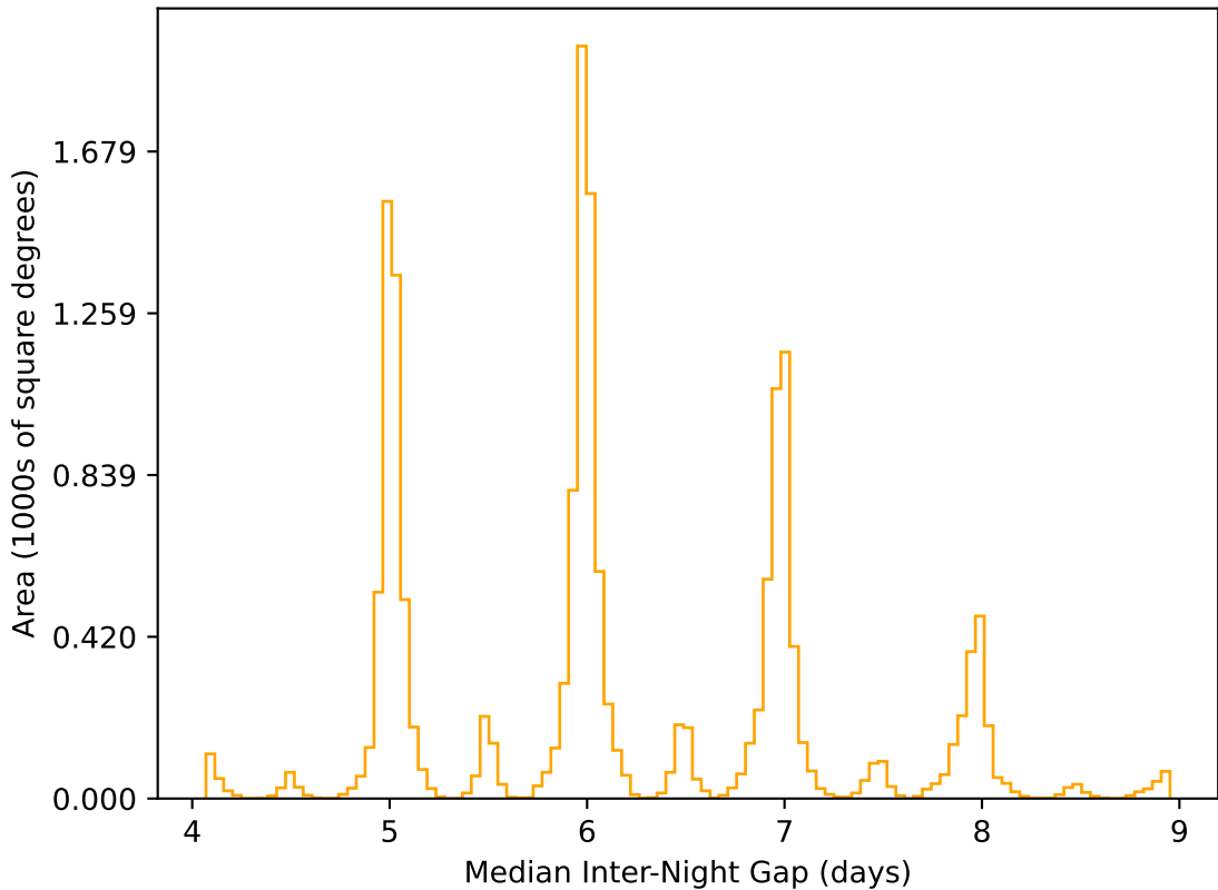
roll_pause_mjdp60_v3.4_10yrs WFD r band: Median Inter-Night Gap
