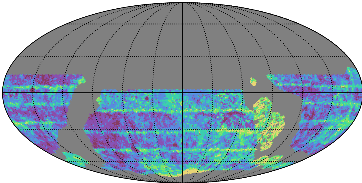
roll_pause_mjdp60_v3.4_10yrs WFD i band: Median Inter-Night Gap
