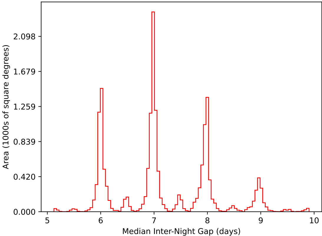
roll_pause_mjdp60_v3.4_10yrs WFD i band: Median Inter-Night Gap
