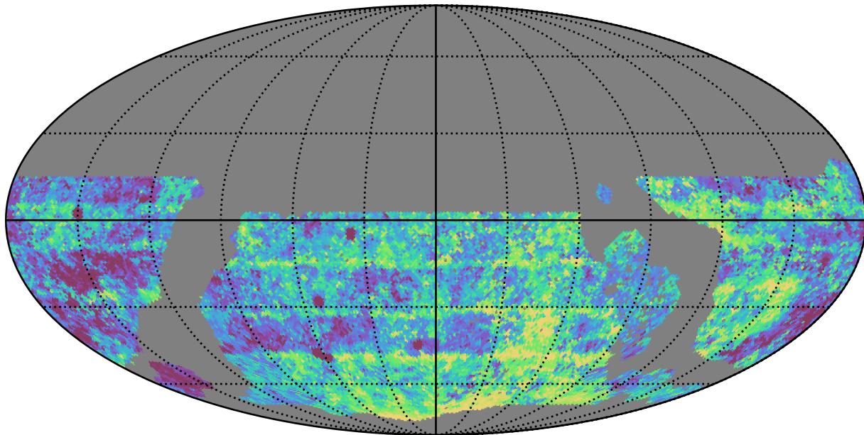
roll_pause_mjdp60_v3.4_10yrs WFD g band: Median Inter-Night Gap
