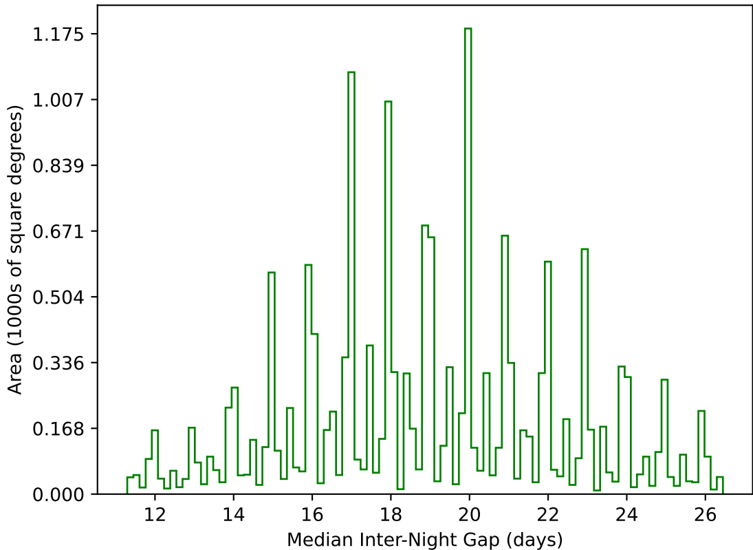
roll_pause_mjdp60_v3.4_10yrs WFD g band: Median Inter-Night Gap
