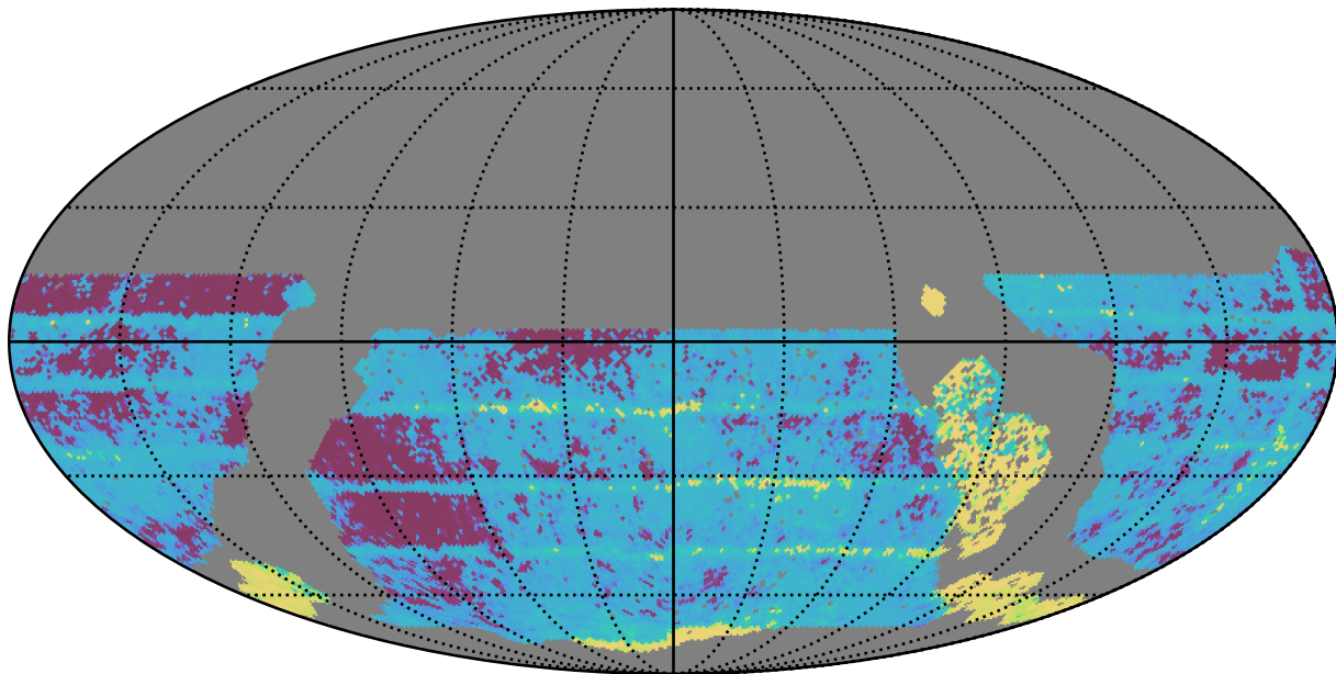
roll_pause_mjdp60_v3.4_10yrs WFD all bands: Median Inter-Night Gap
