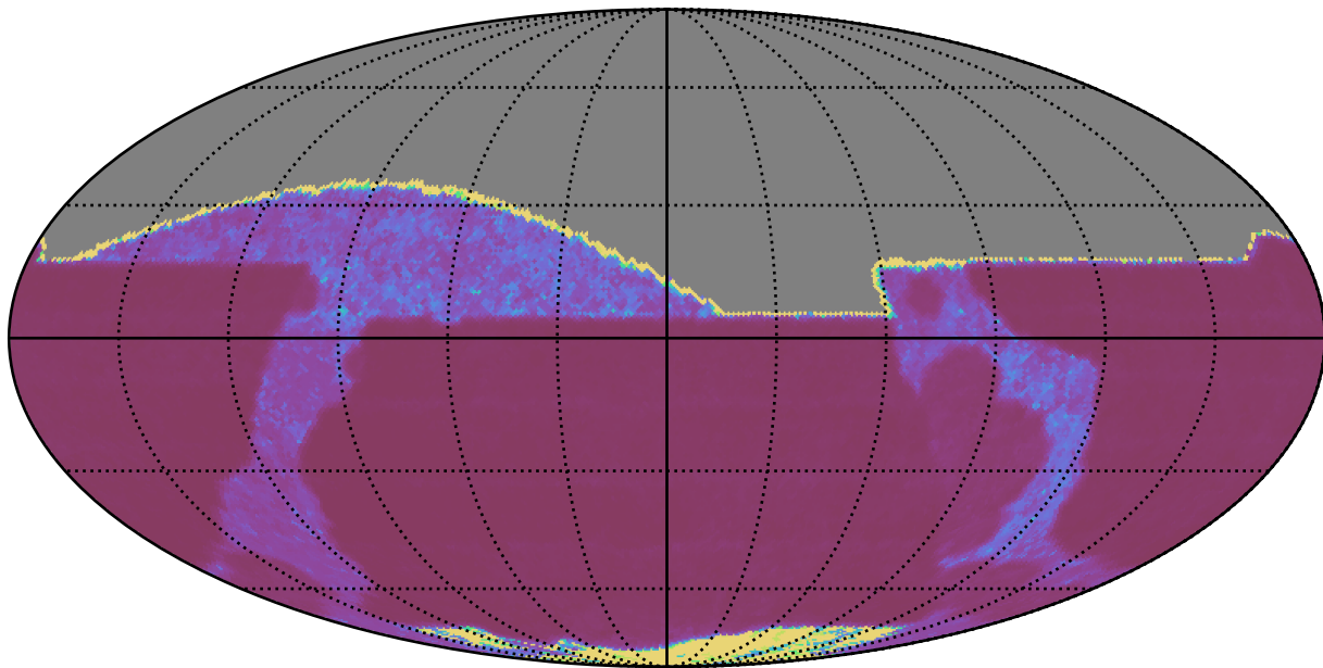
roll_pause_mjdp60_v3.4_10yrs All sky z band: Median Inter-Night Gap
