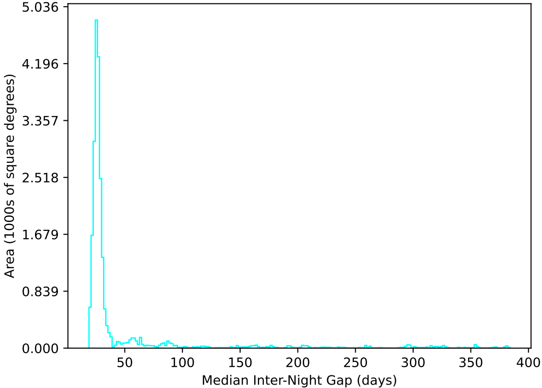
roll_pause_mjdp60_v3.4_10yrs All sky u band: Median Inter-Night Gap
