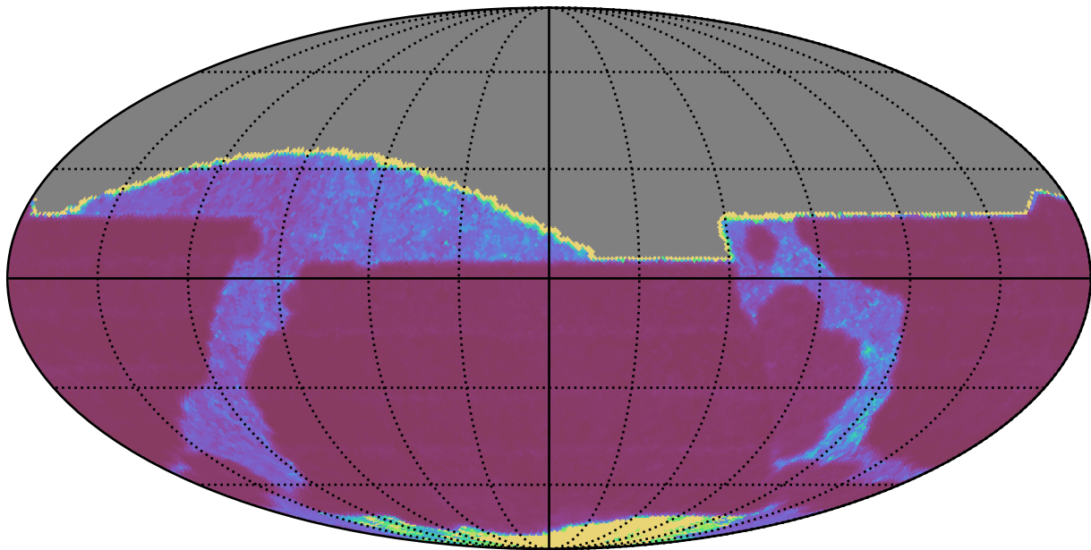
roll_pause_mjdp60_v3.4_10yrs All sky i band: Median Inter-Night Gap
