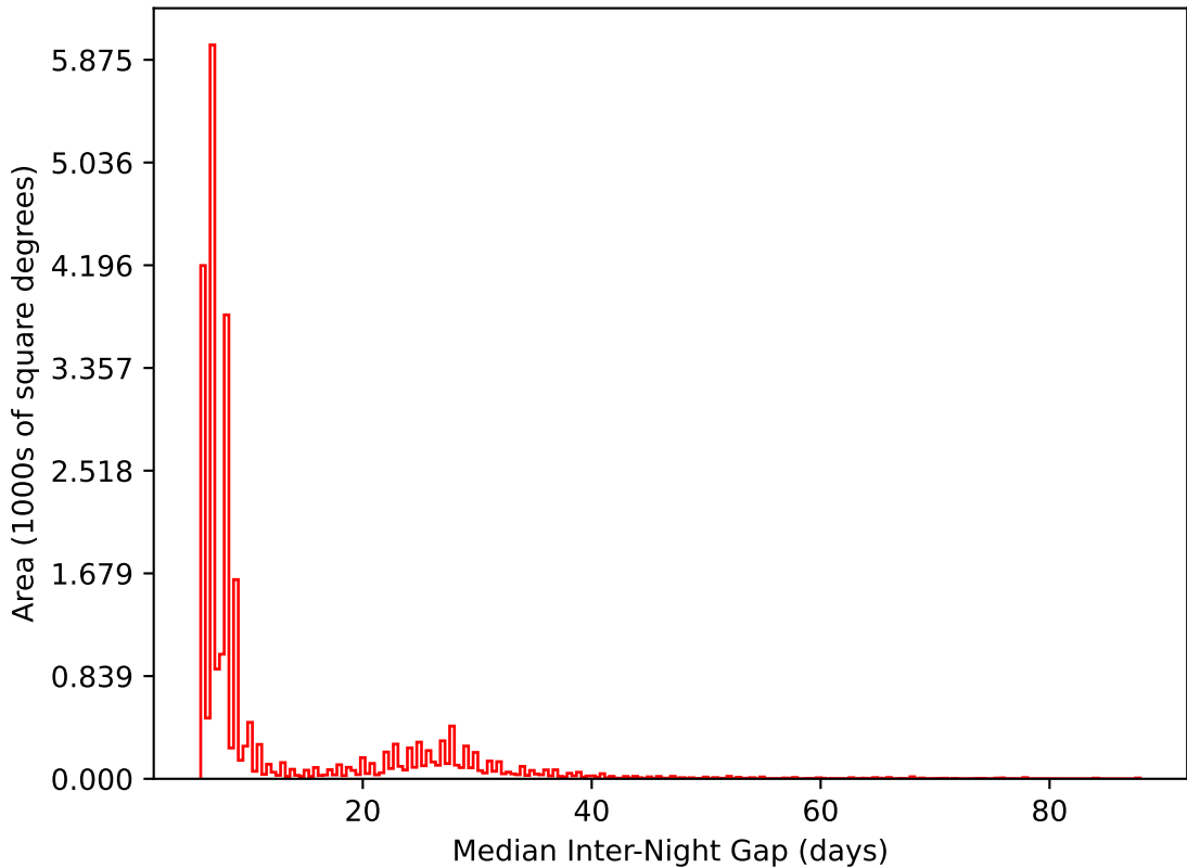
roll_pause_mjdp60_v3.4_10yrs All sky i band: Median Inter-Night Gap
