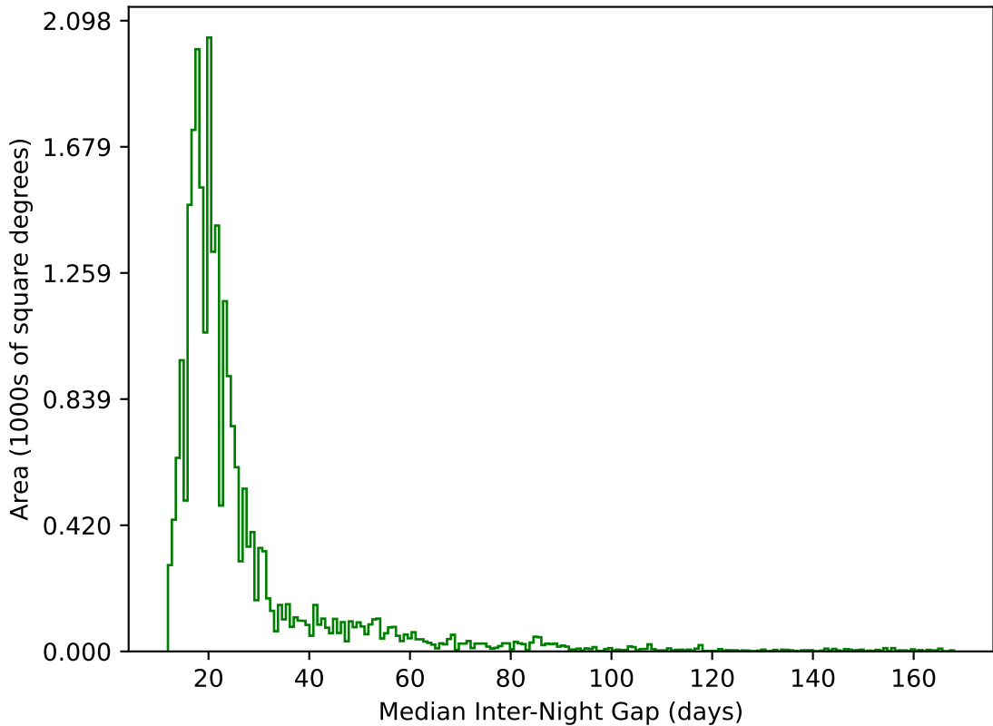
roll_pause_mjdp60_v3.4_10yrs All sky g band: Median Inter-Night Gap
