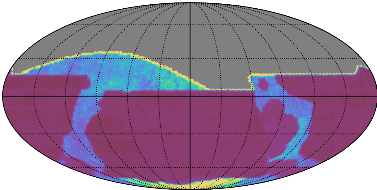
roll_pause_mjdp60_v3.4_10yrs All sky all bands: Median Inter-Night Gap
