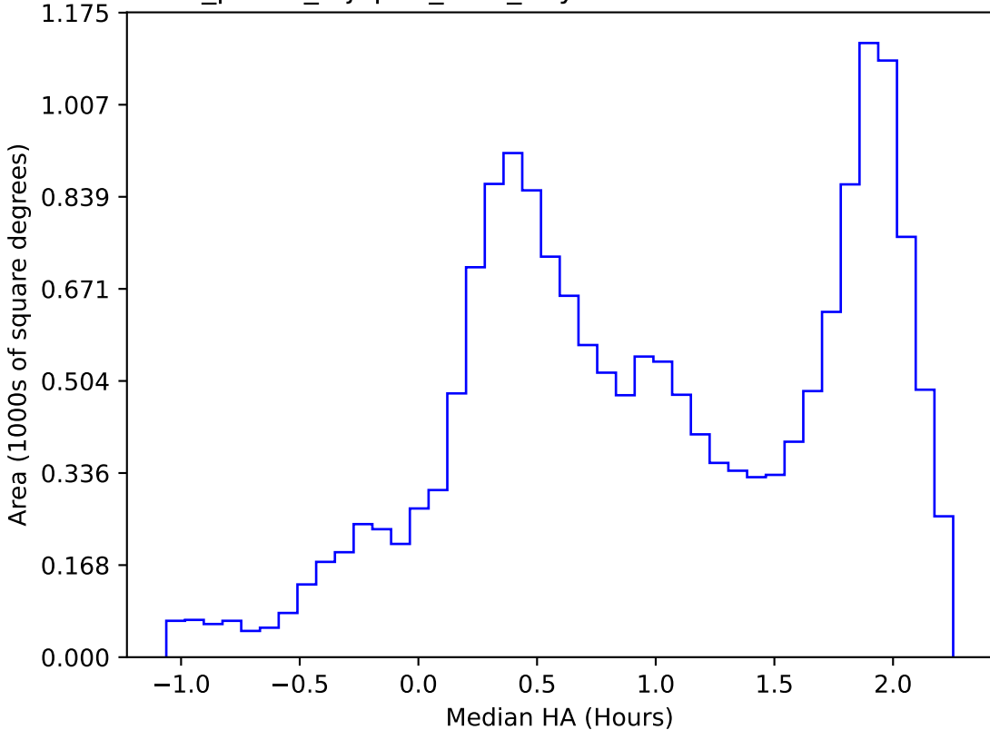
roll_pause_mjdp60_v3.4_10yrs WFD z band: Median HA
