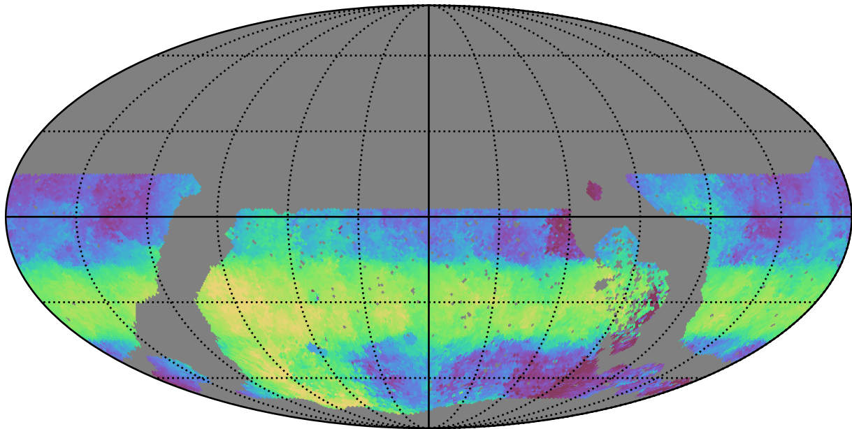
roll_pause_mjdp60_v3.4_10yrs WFD u band: Median HA
