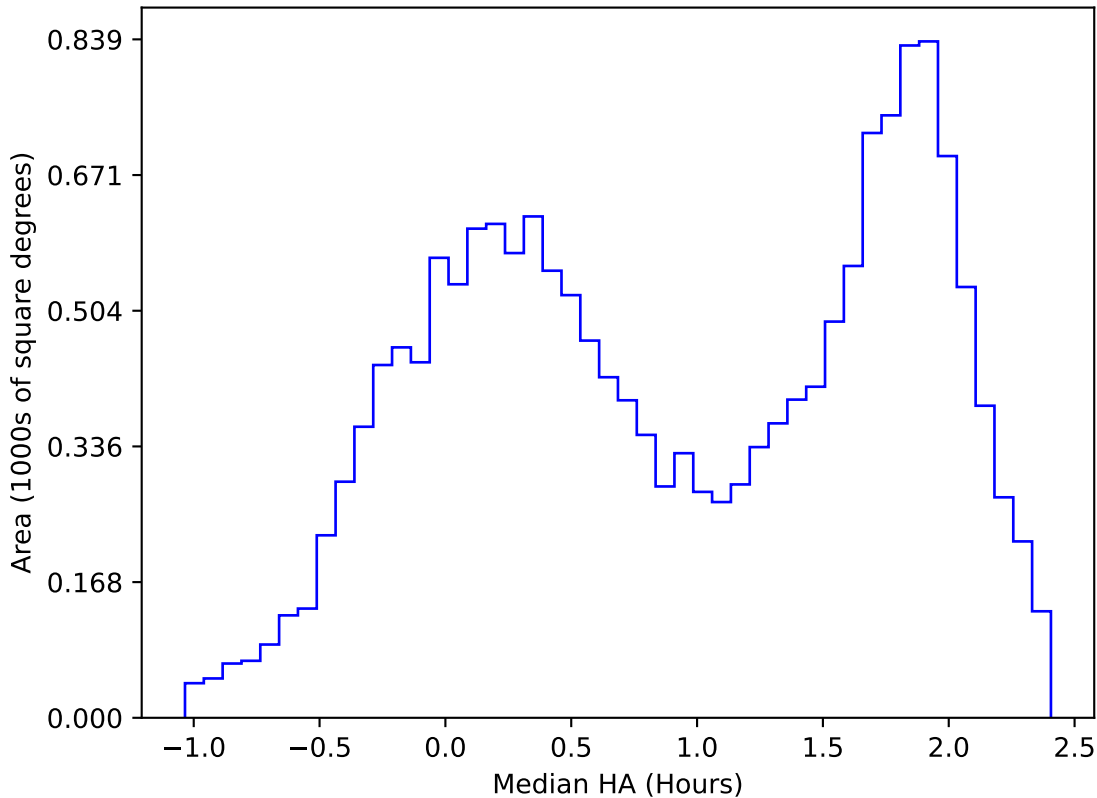
roll_pause_mjdp60_v3.4_10yrs WFD u band: Median HA
