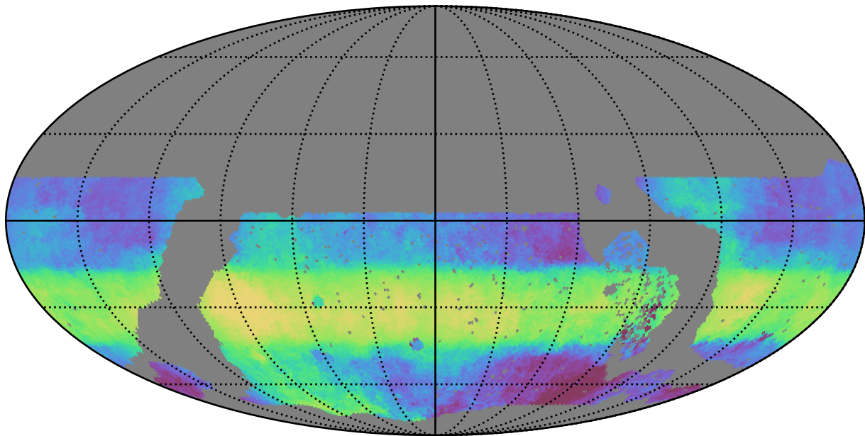
roll_pause_mjdp60_v3.4_10yrs WFD r band: Median HA
