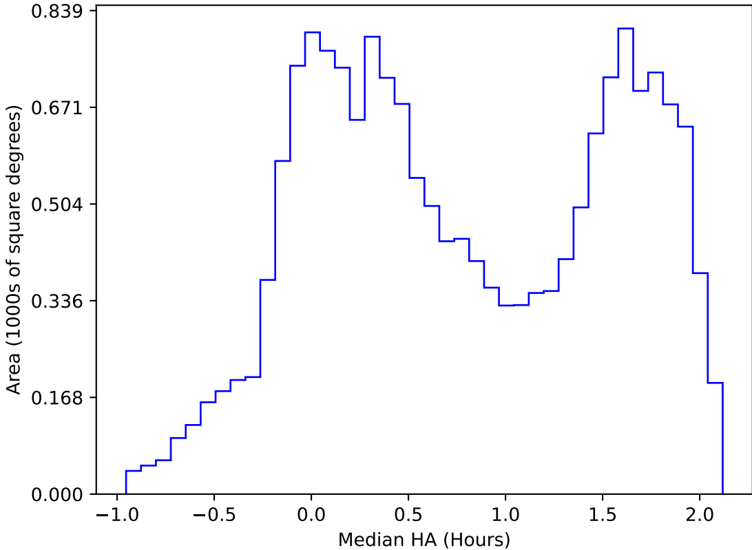
roll_pause_mjdp60_v3.4_10yrs WFD r band: Median HA
