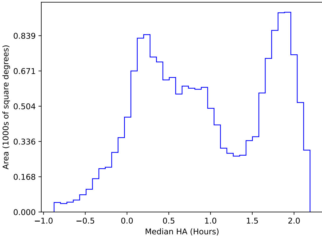
roll_pause_mjdp60_v3.4_10yrs WFD i band: Median HA
