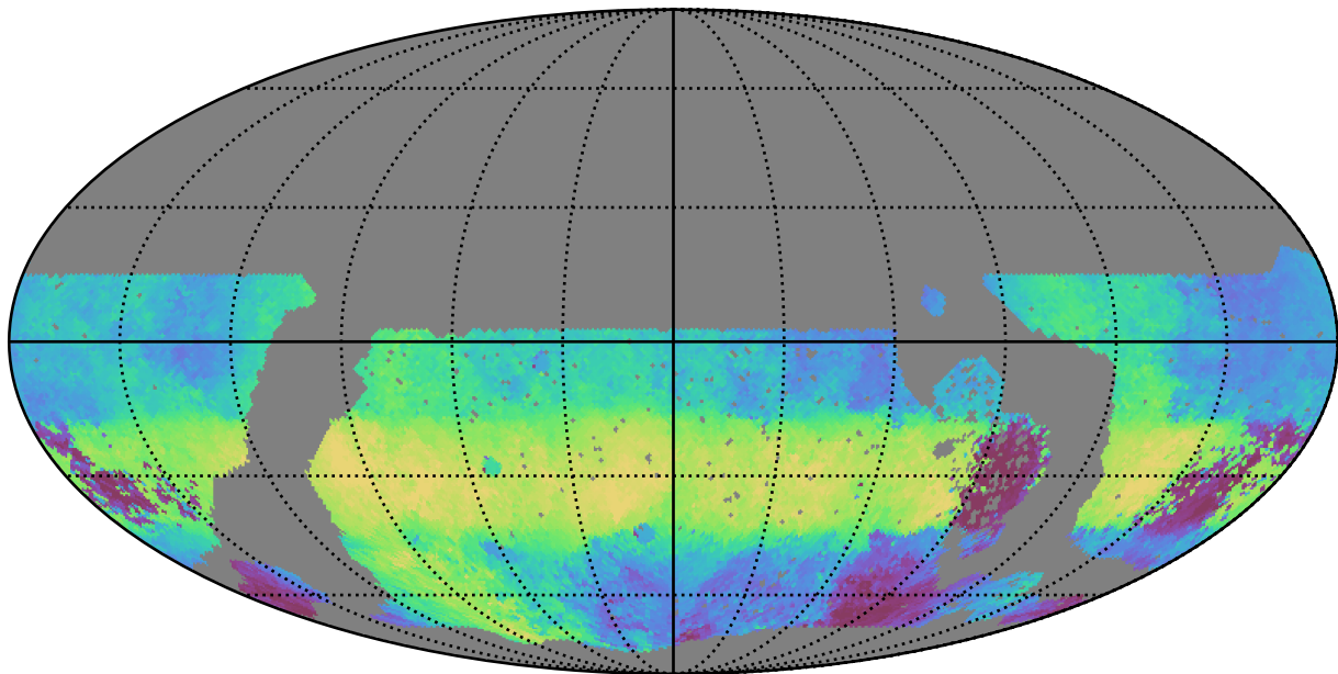
roll_pause_mjdp60_v3.4_10yrs WFD g band: Median HA
