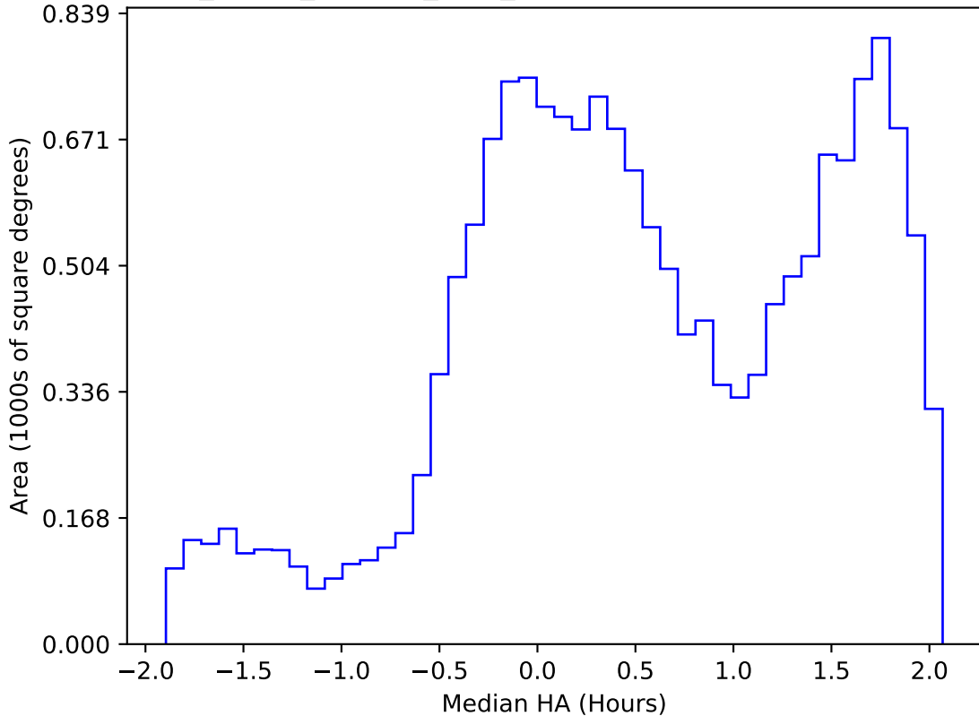
roll_pause_mjdp60_v3.4_10yrs WFD g band: Median HA
