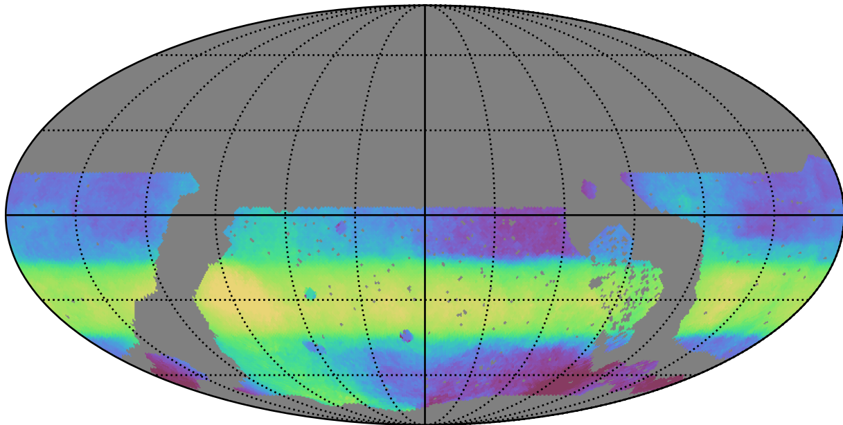
roll_pause_mjdp60_v3.4_10yrs WFD all bands: Median HA
