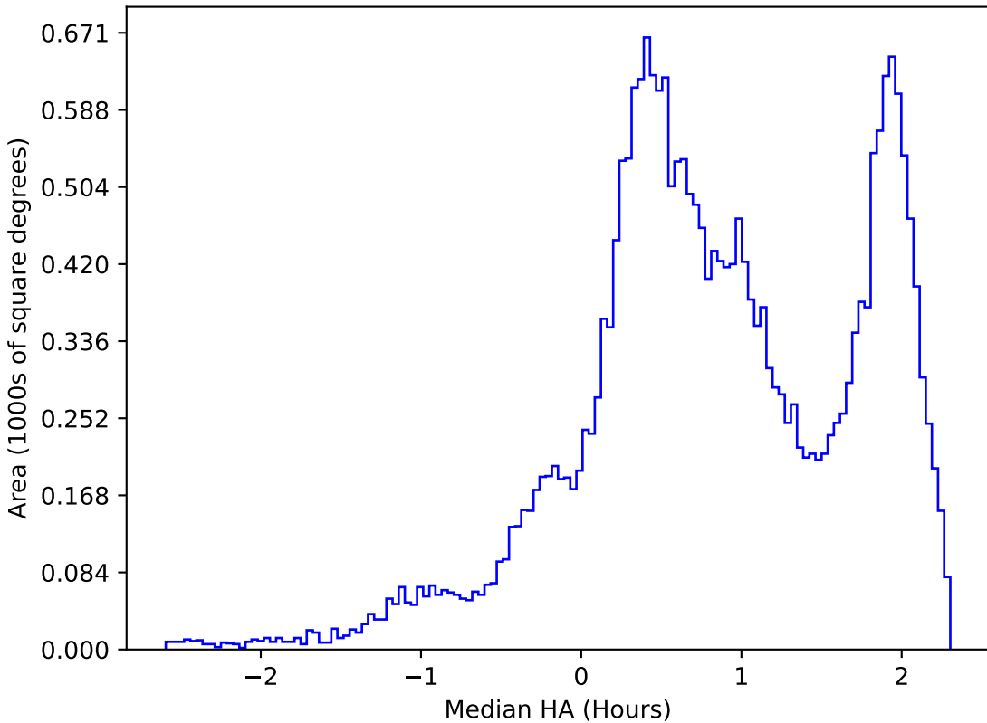
roll_pause_mjdp60_v3.4_10yrs All sky z band: Median HA
